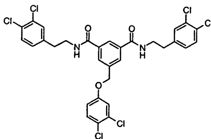
Compound # 19
